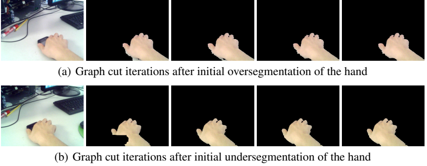
Fig. 3. Given a pair of images, the hand is iteratively segmented using graph cuts. Then, stereo matching, followed by bilateral filtering, is performed on the segmented images to generate point clouds which are used as inputs for recognition.
