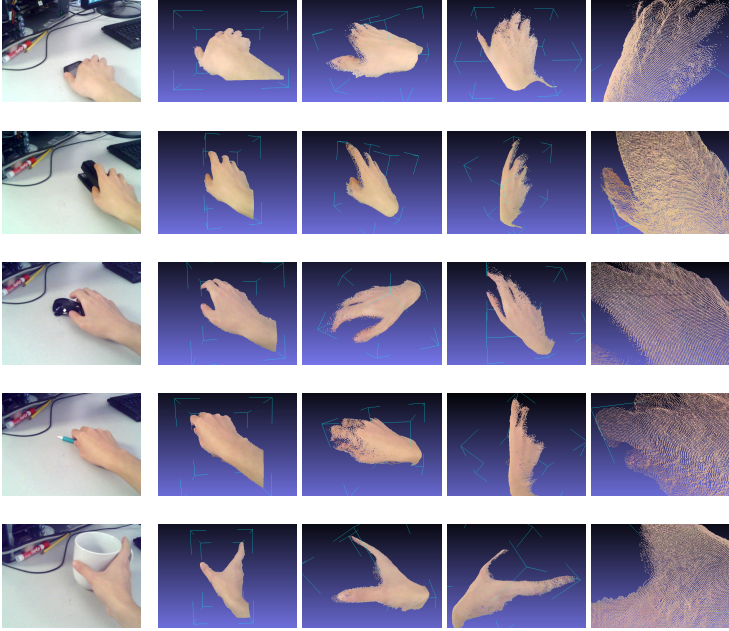
Fig. 6. Visualizations of the reconstructed dense 3D point clouds of the grasping hand along with original video frames. From left to right, each row presents the original video frame and the dense 3D point cloud of the grasping hand viewed from different angles and at different scales.
