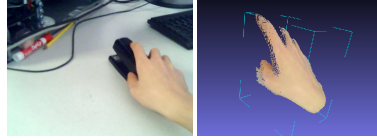
Fig. 12. This frame of a stapler was incorrectly classified as an iPhone. In appearance, the stapler in this frame looks like an iPhone. Because the grasping gesture of the hand is totally different when people grasp an iPhone, factoring the 3D features of the grasping hand again helped to recognize it correctly.
